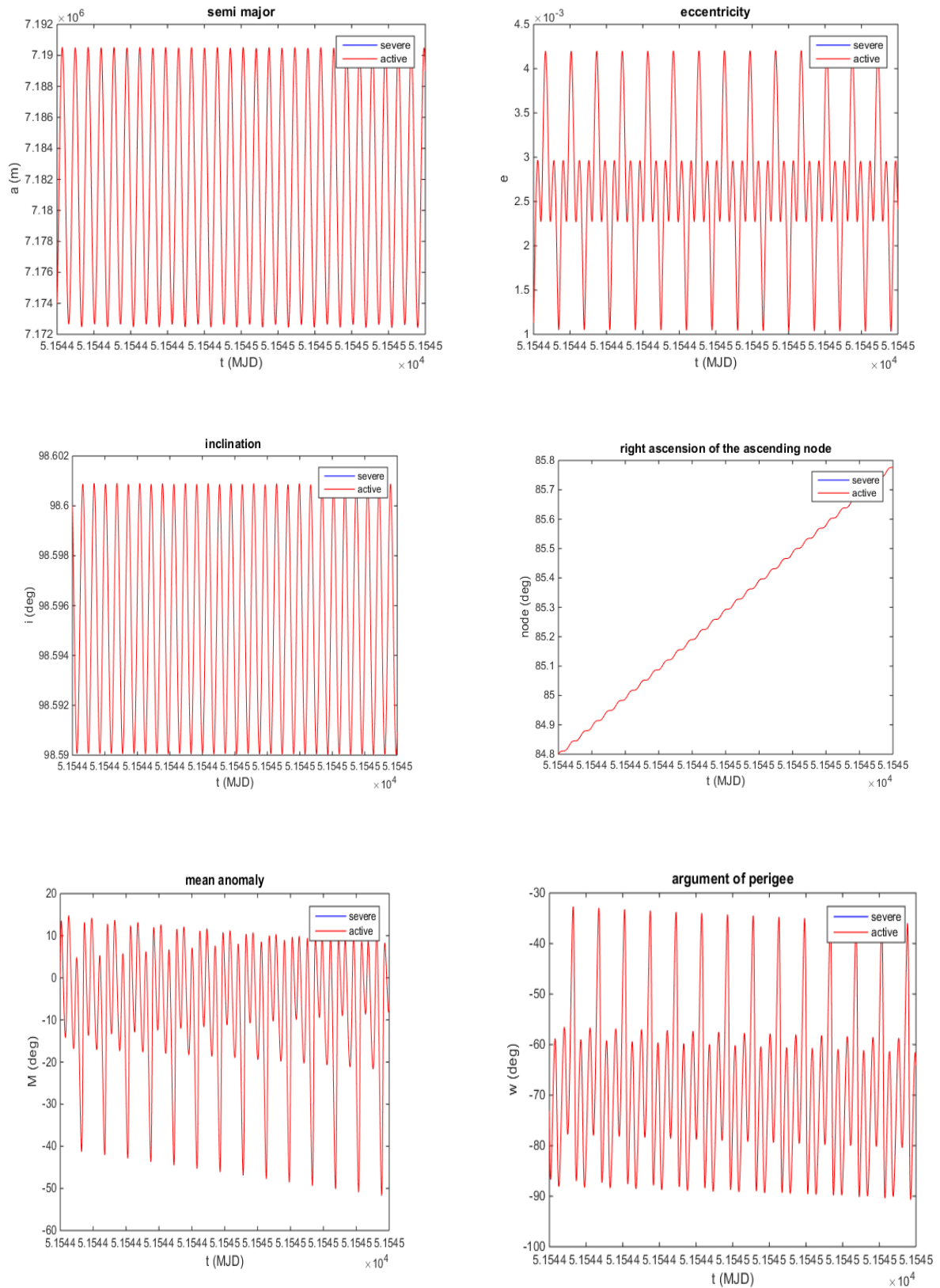
Fig(1) orbital elements for NOAA 15 satellite under atmospheric perturbation in two solar condition (active and severe storm solar condition)
