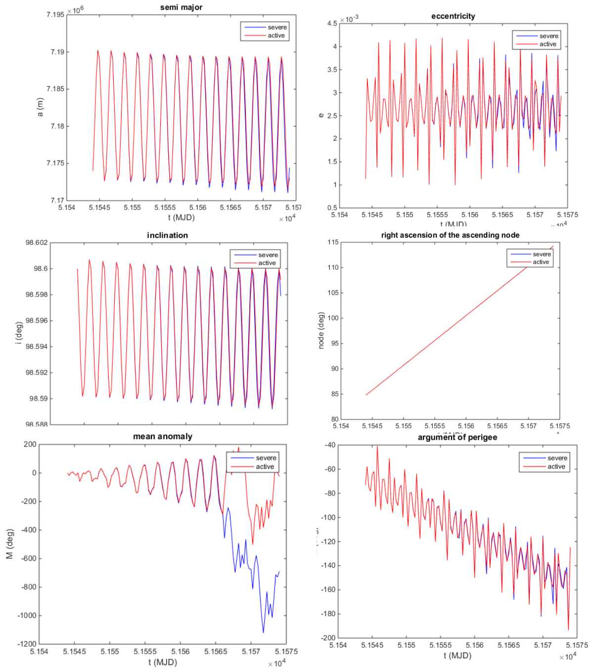
Fig(4) orbital elements for NOAA 15 satellite under atmospheric perturbation in two solar condition (active and severe storm solar condition for 30 days
