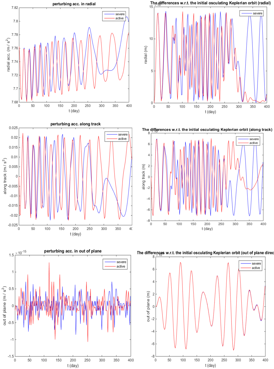
Figure (9) the difference w.r.t. the initial osculating Keplerian orbit for 400 days
