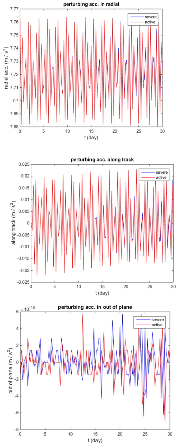
Figure (5) acceleration component for NOAA for 30 days
