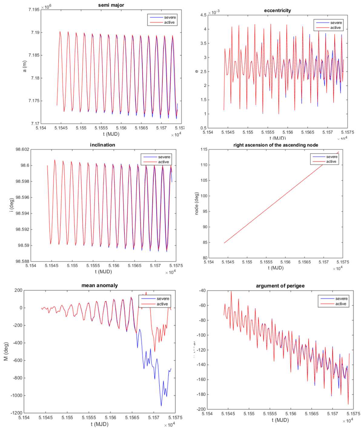
Fig(1) orbital elements for NOAA 15 satellite under atmospheric perturbation in two solar condition (active and severe storm solar condition
